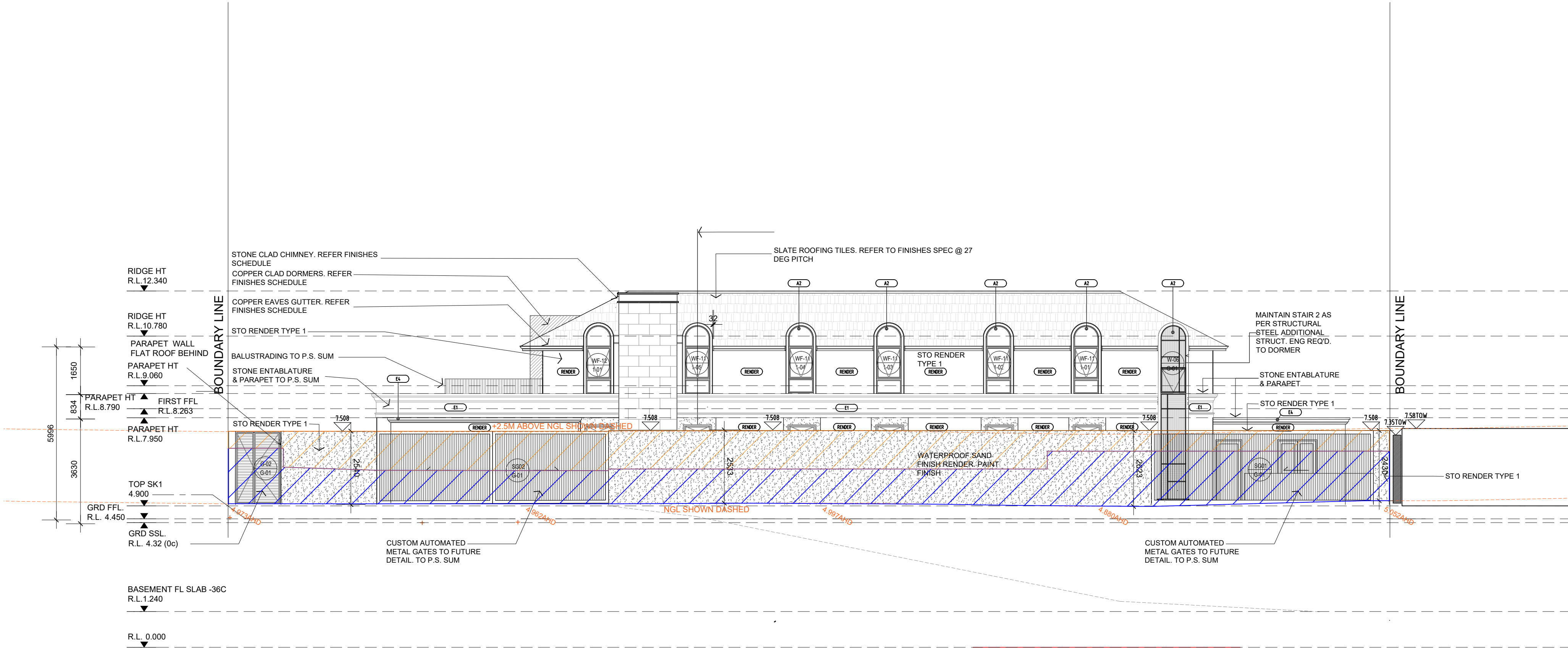
WEST ELEVATION
